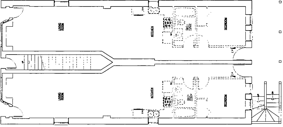
EXISTING FIRST FLOOR PLAN SCALE: 1/4"=1'-0"
