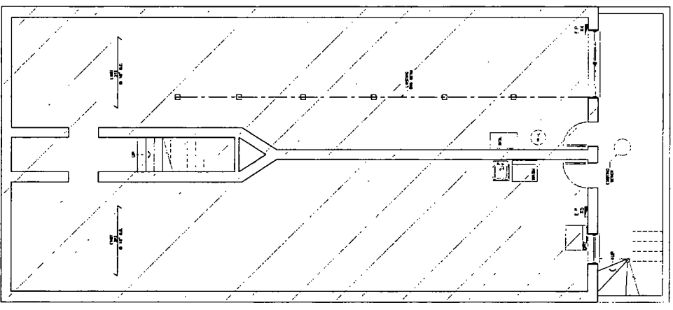
EXISTING BASEMENT PLAN SCALE: 1/4"=1'-0"
