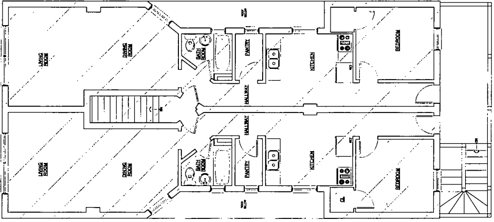
EXISTING SECOND FLOOR PLAN SCALE: 1/4"=1'-0"
