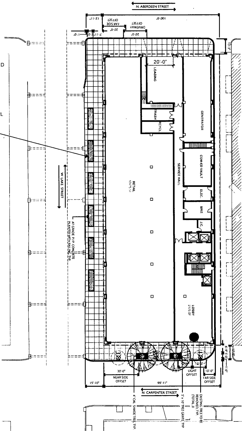
SITE / LANDSCAPE PLAN
