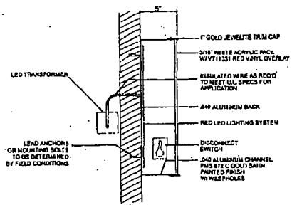
SECTION THRU CHANNEL LETTER - INT
