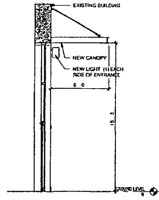
3 CANOPY WALL SECTION 2 LEVEL 1 - ENLARGED PLAN SOUTH ENTRANCE
