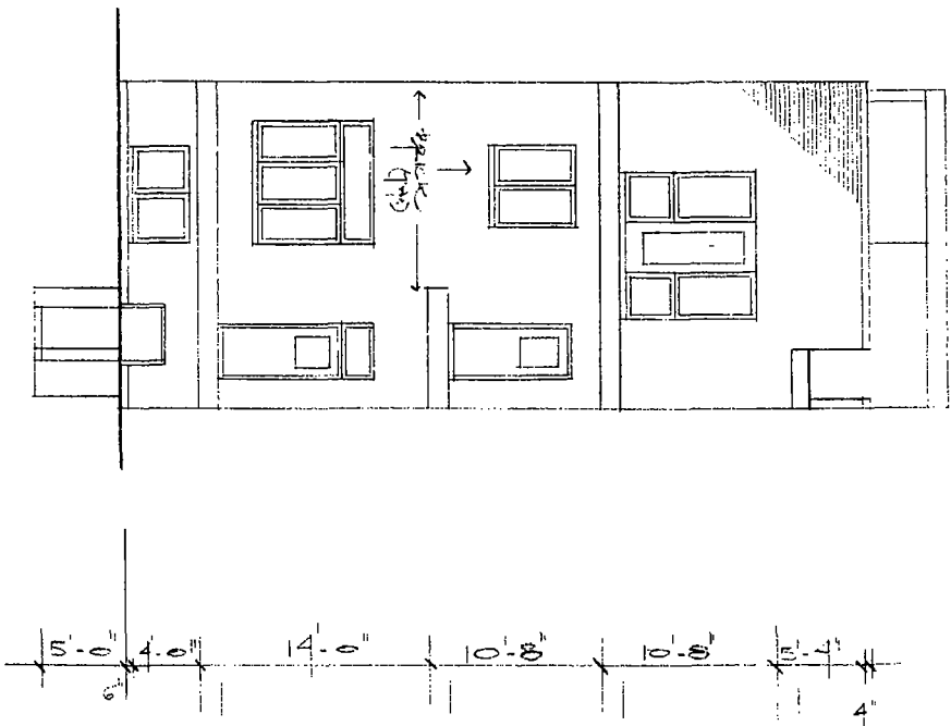
○ PARK ELEVATION 1/8" = 1'-0"
