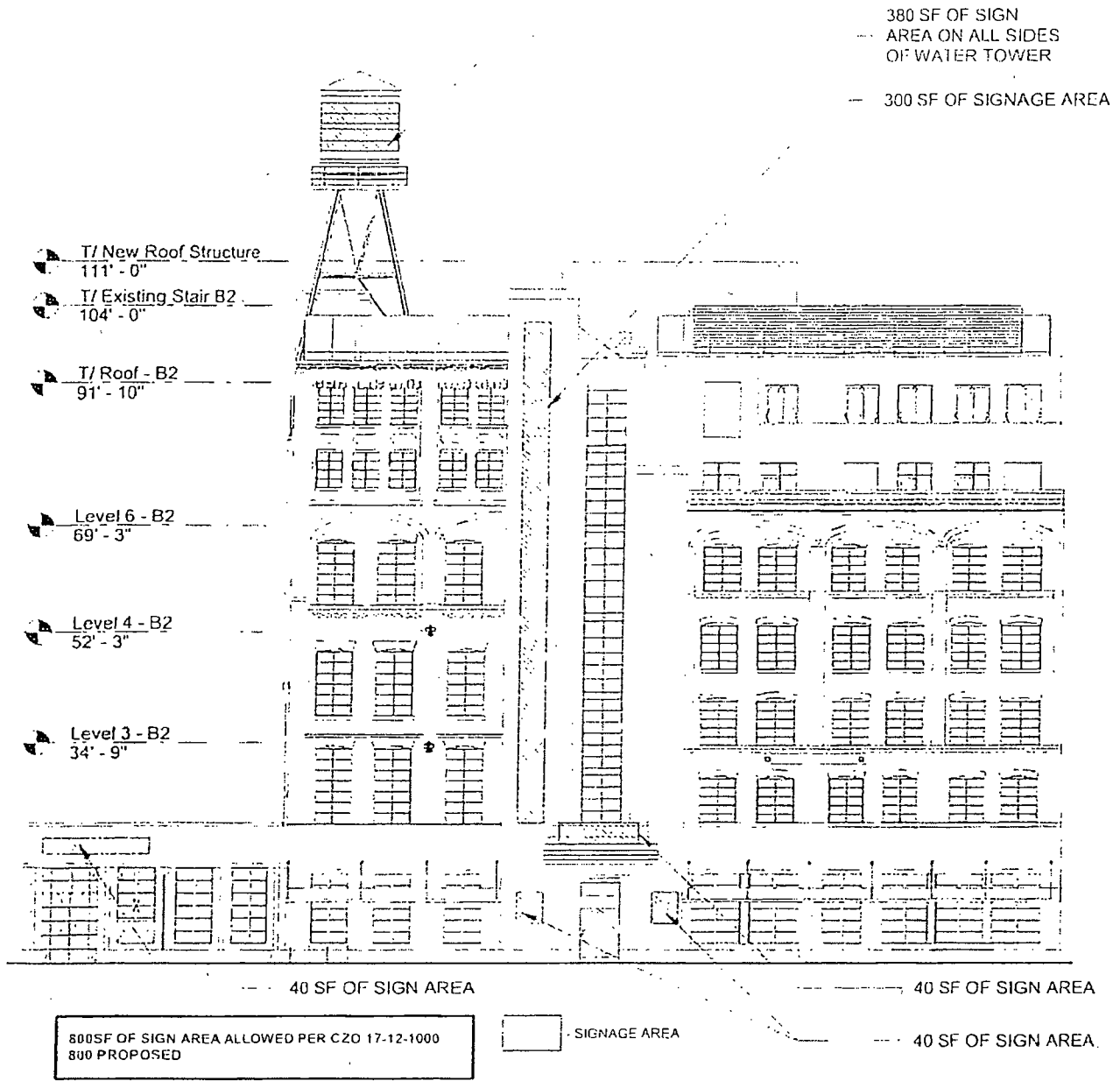
1 West Elevation - Sub Area A Signage Area 3/64" = 1'-0"
