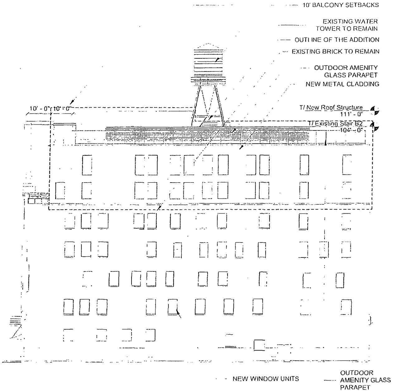
1 South Elevation - Sub Area A 3/64" = 1'-0"
