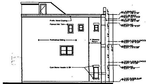
Typical Side Elevation
