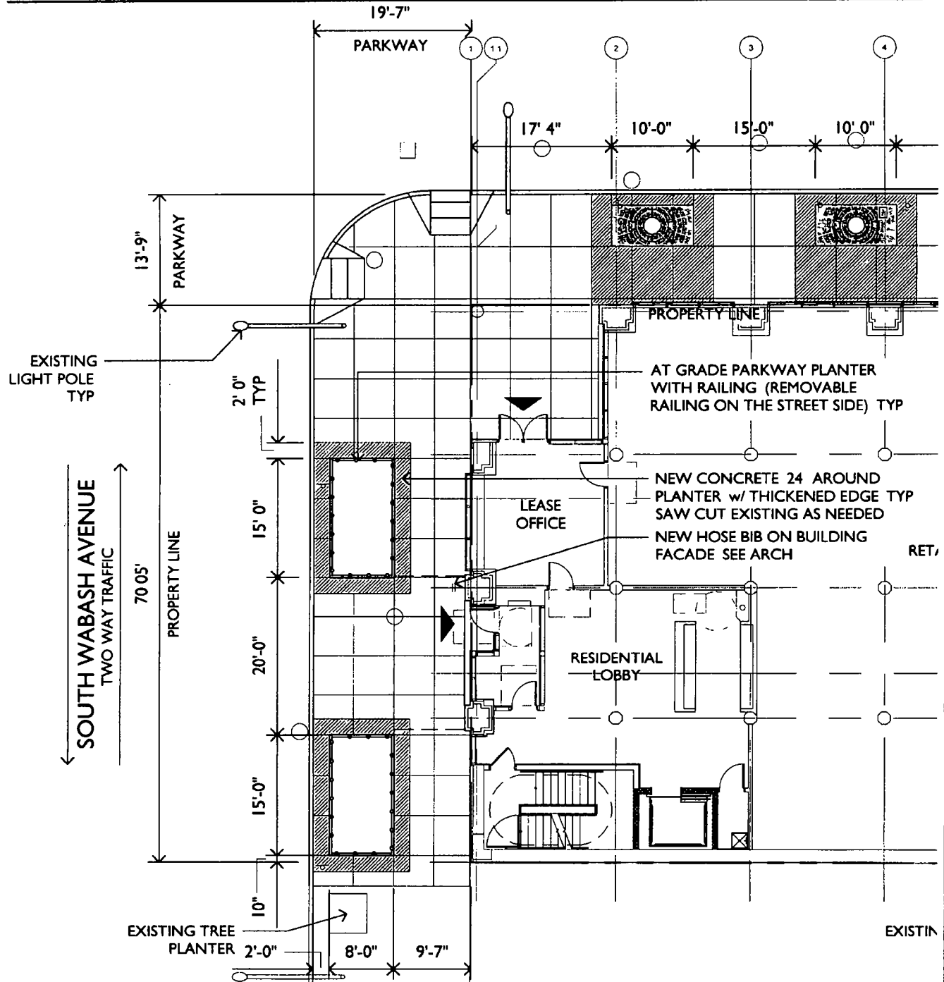
GROUND FLOOR HARDSCAPE PLAN SCALE 1/16" = 1'-0"
