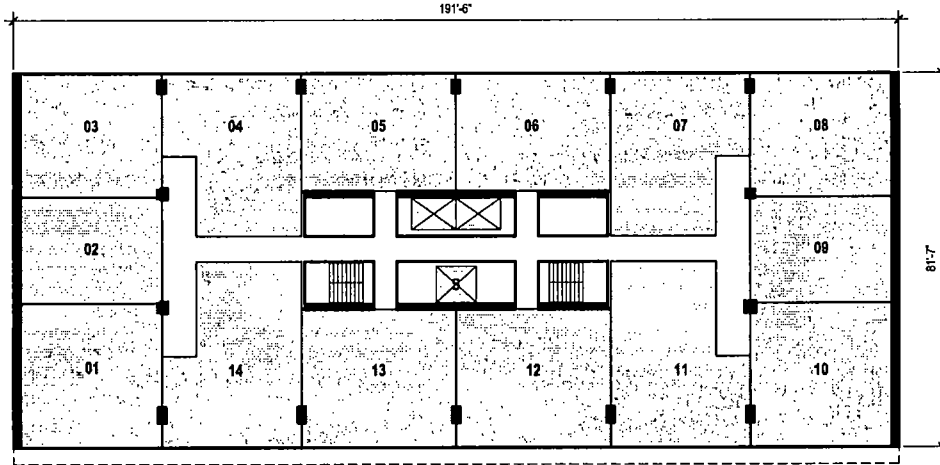
POTENTIAL LAYOUT WITH STANDARD DWELLING UNITS AND EFFICIENCIES Note: Edge of building and balcony layout varies per floor.
