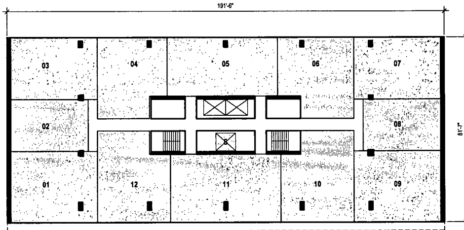
POTENTIAL LAYOUT WITH STANDARD DWELLING UNITS Note: Edge of building and balcony layout varies per floor.
