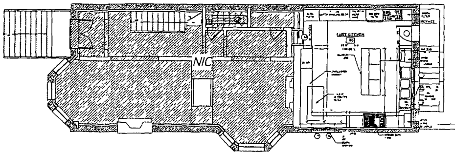
1 FIRST FLOOR PLAN 1/4" = 1'-0"
