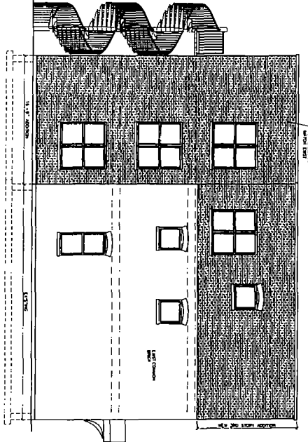
EAST ELEVATION
