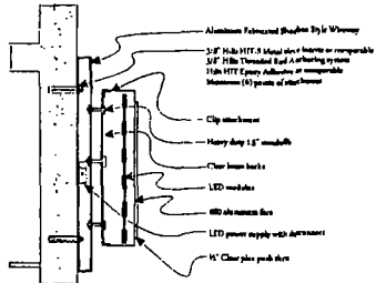
Detail - Section thru
