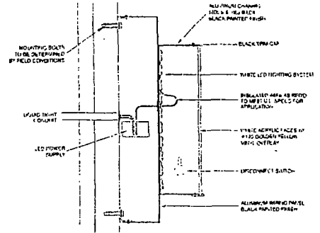
PANEL MOUNT INTERNALLY ILLUM. CHANNEL LTR.
