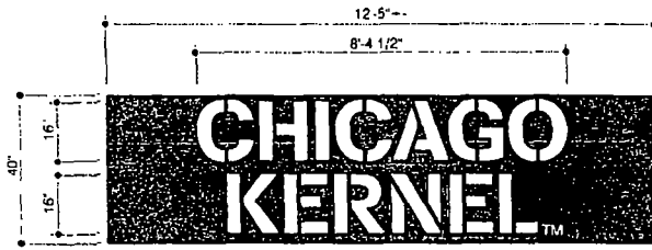
INDIVIDUAL INT. LED ILLUMINATED LETTER DISPLAY 3/8" = 1'-0"
