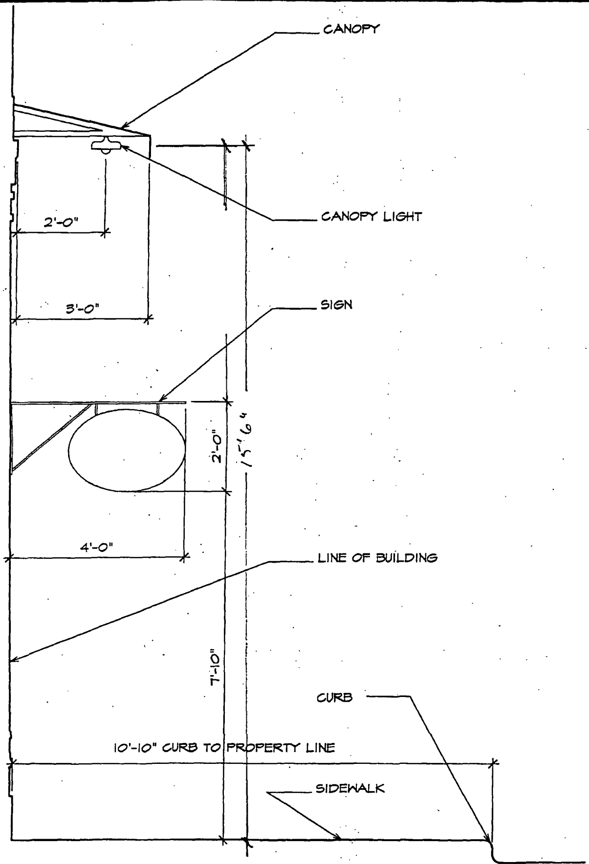
(A) SIDEWALK ELEVATION (A1) 1/2" = 1'-0"
