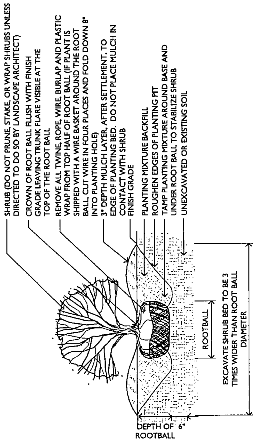
2 SHRUB INSTALLATION DETAIL SCALE: NOT TO SCALE
