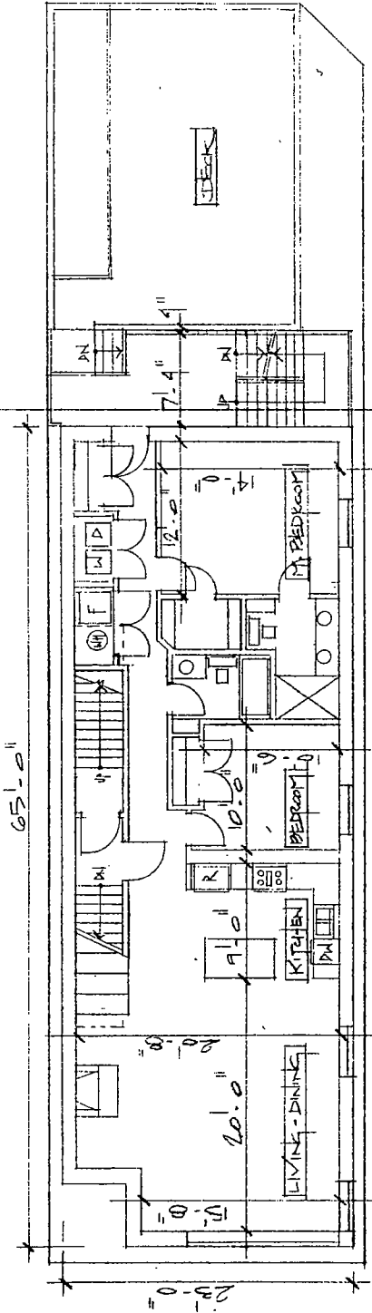
2 nd Floor PLAN 1470 S.F. 1/8" = 1'-0"
