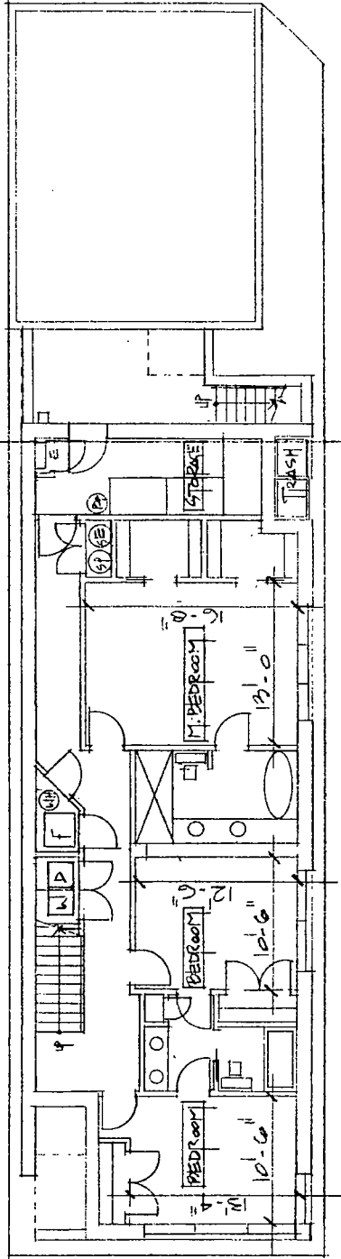
○ BASEMENT Floor PLAN 1/8" = 1'-0"
