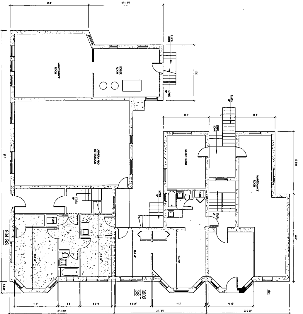
1 BSMT FLOOR PLAN 1/8" = 1'-0"
