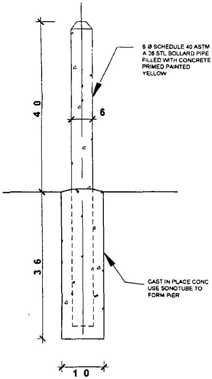
2 BOLLARD DETAIL SCALE 1/2 1-0
