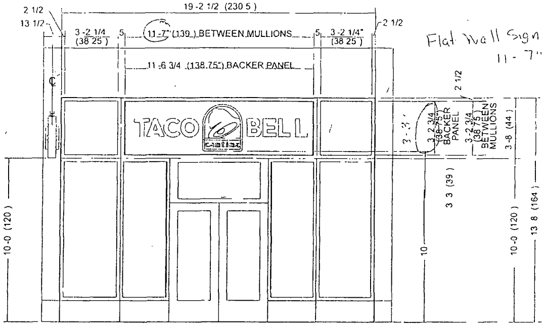
STOREFRONT ELEVATION SCALE 1/4"=1'-0
