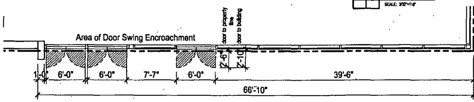
3 Plan at Partial West Elevation SCALE: 3/32"=1'-0"
