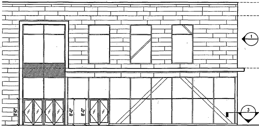
2 Partial West Elevation SCALE: 3/32"=1'-0"
