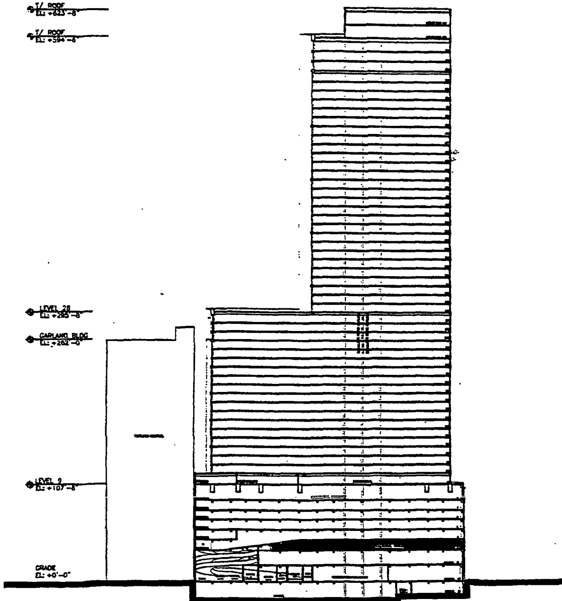
BUILDING SECTION A-A - LOOKING WEST
