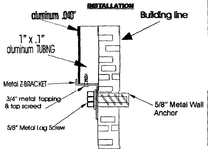
All joints are to be 100 % screwed
