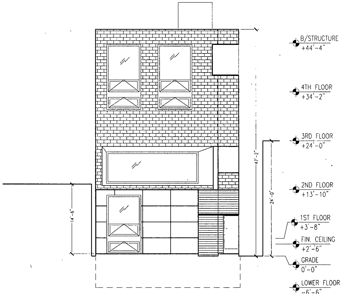
02 South Elevation SCALE: 1/8"=1'-0"
