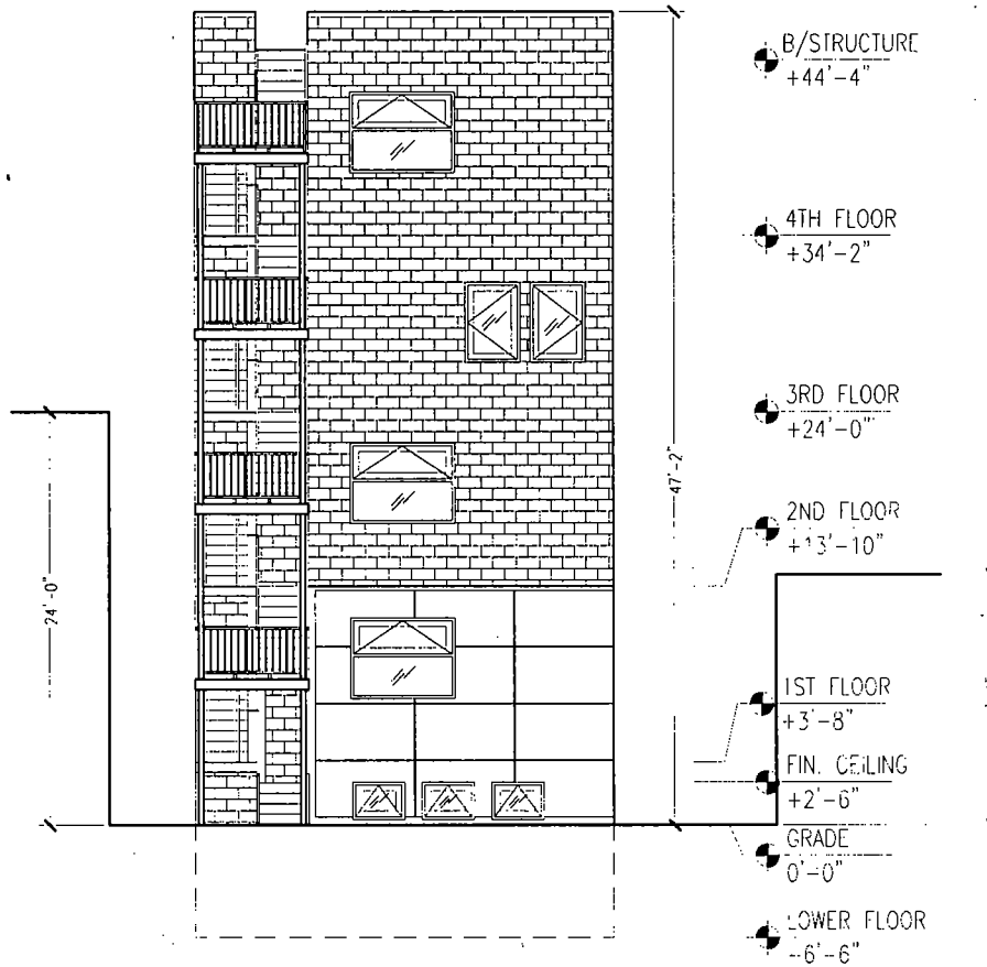
03 North Elevation SCALE: 1/8"=1'-0"
