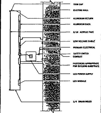
Standard Face Lit LED Illuminated w/ Raceway
