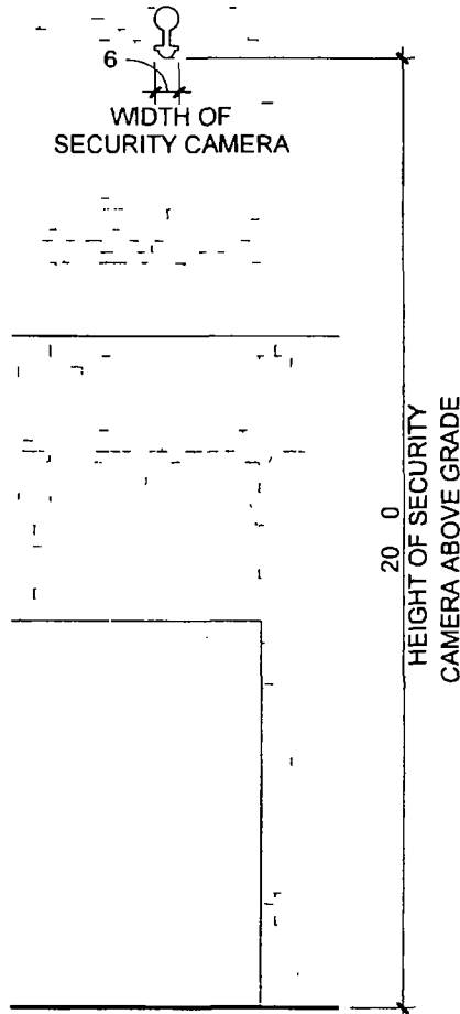
SECURITY CAMERA ELEVATION, TYP FOR CAMERAS 1, 2, 3 & 4*
