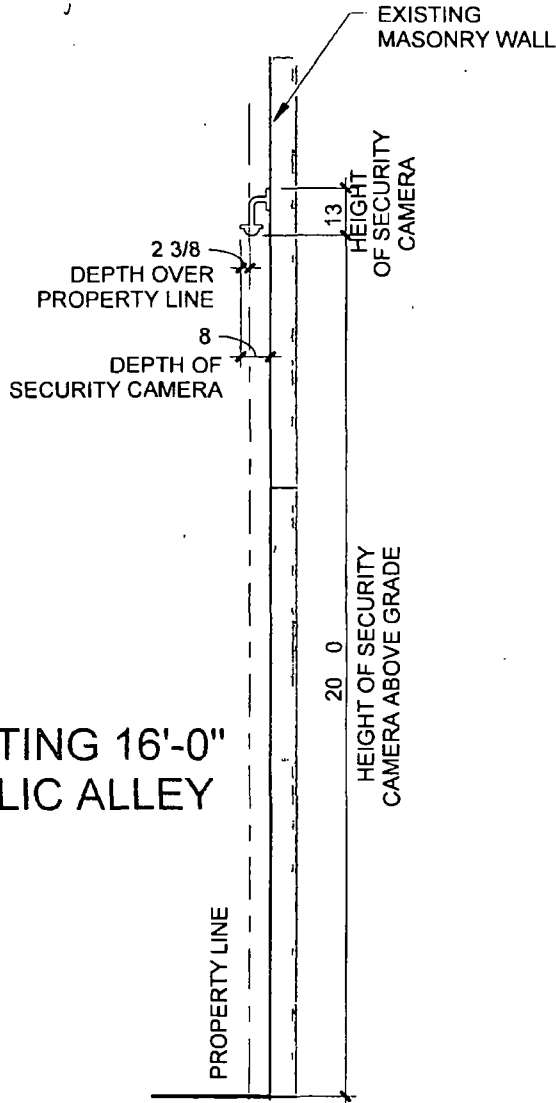
SECURITY CAMERA SECTION, TYP FOR CAMERAS 1, 2, 3 & 4*
