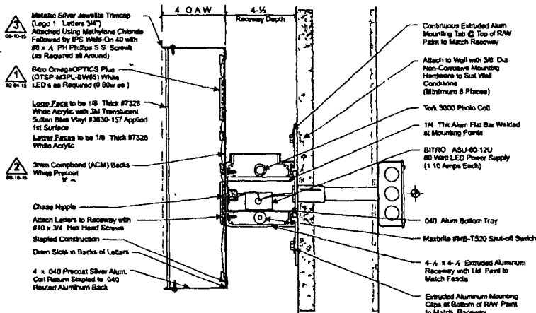
SECTION Scale 3 = 1-0
