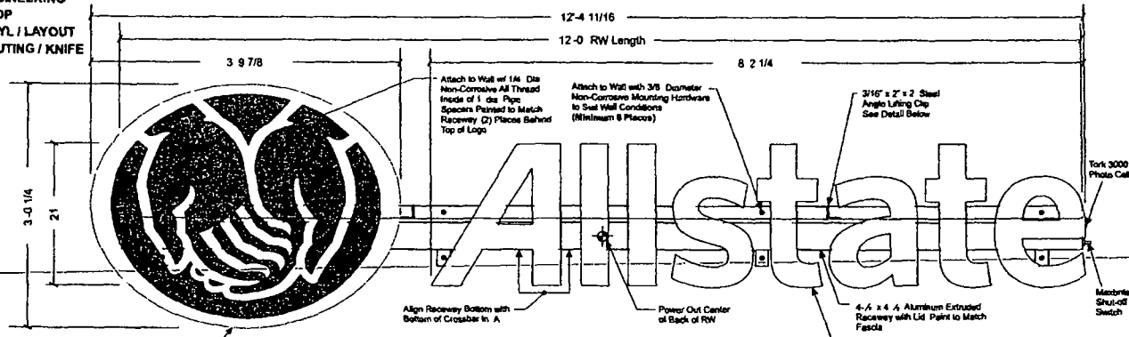
ALST CL RW WEL 21 FRONT ELEVATION Scale 1 = 1-0
