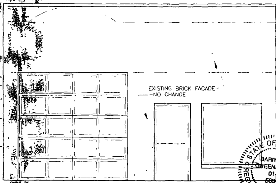
EXISTING SOUTH ELEVATION SCALE 3/4" = 1'-0"
