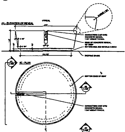
4 PRECAST CONCRETE BLOCK TYPE 'B' - LARGE 12" x 12"
