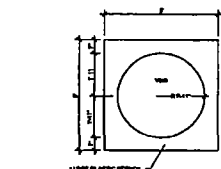
3 STENCIL TYPE 'B' - LARGE PAINTED CIRCLES 12" x 12"
