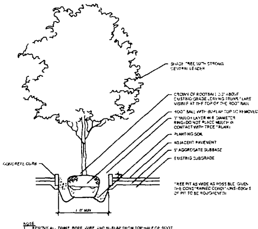
2 SHADE TREE IN RAISED PLANTER SECTION NOT TO SCALE
