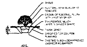
4 SHRUB PLANTING SECTION NOT TO SCALE
