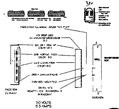
TYPICAL LED ILLUMINATED CHANNEL LETTER MOUNTED TO W/RACEWAY
