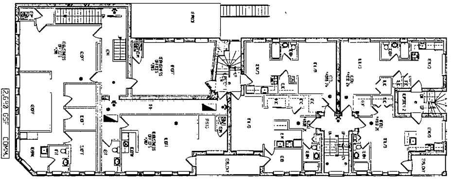
3) 3RD FLOOR PLAN SCALE: 1/8" = 1'-0" DATE: 12/17/2020
