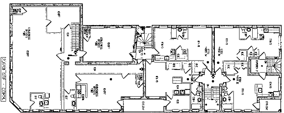
4) 4TH FLOOR PLAN SCALE: 1/8" = 1'-0" DATE: 12/17/2020
