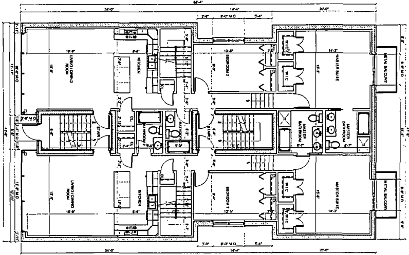
1st Floor Plans (Duplex)
