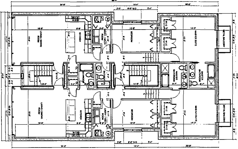
2nd - 4th Floor Plans (Simpler)
