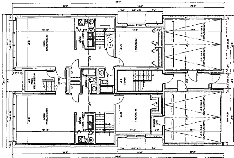
Basement Floor Plans (Duplex)
