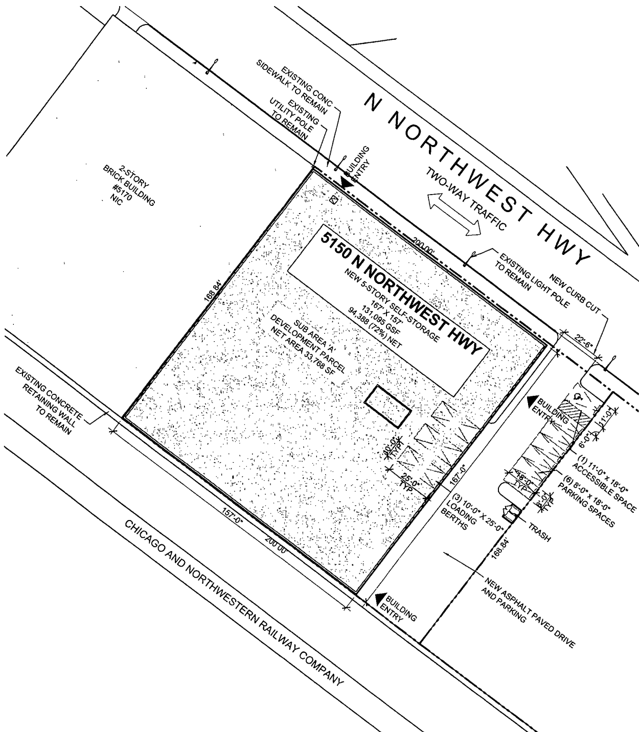
SITE PLAN SUB AREA 'A'
