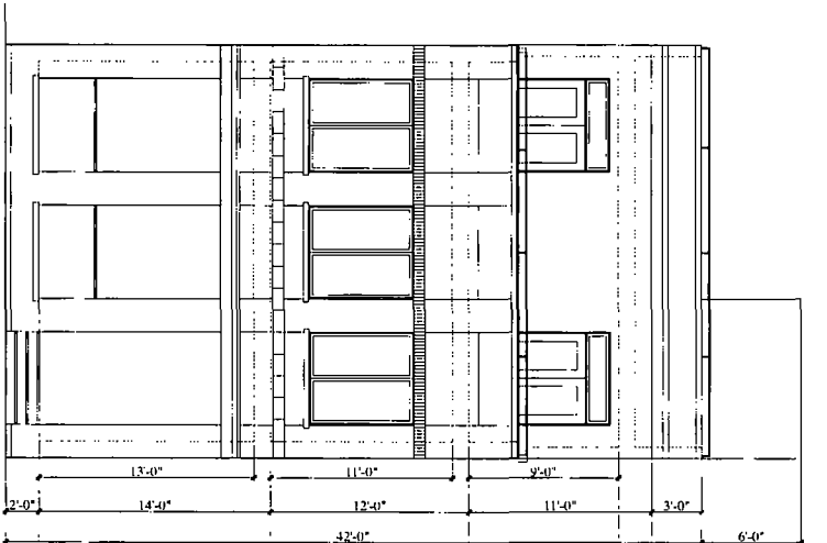
Front (South) Elevation 1/8" = 1'-0"
