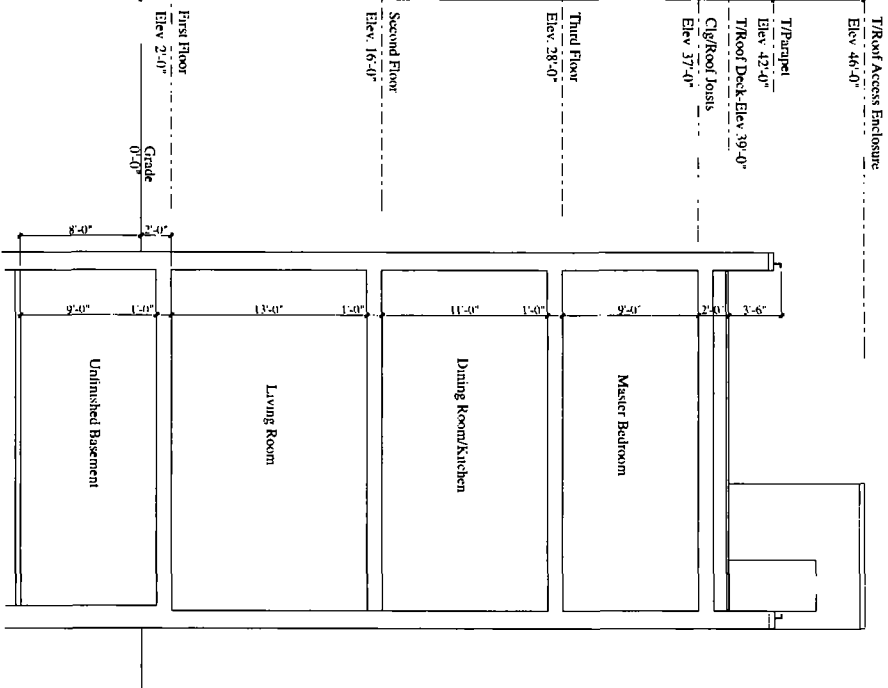
Building Section 1/8" = 1'-0"
