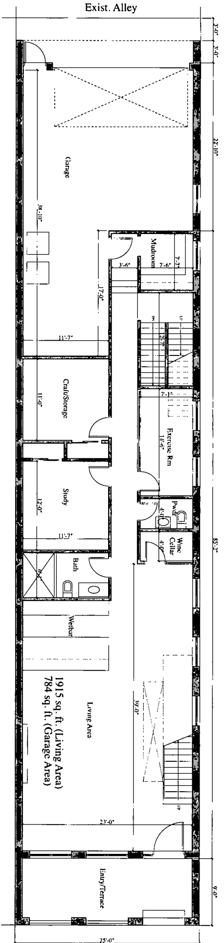
Proposed First Floor Plan
