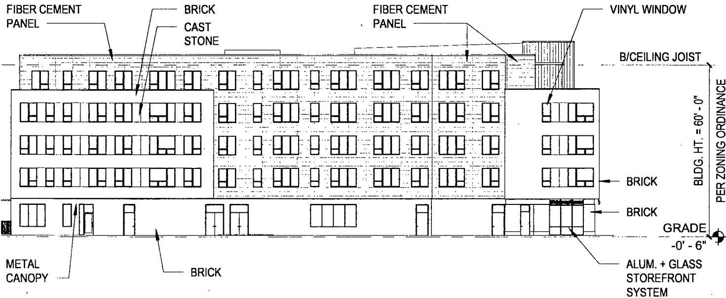
EAST ELEVATION
