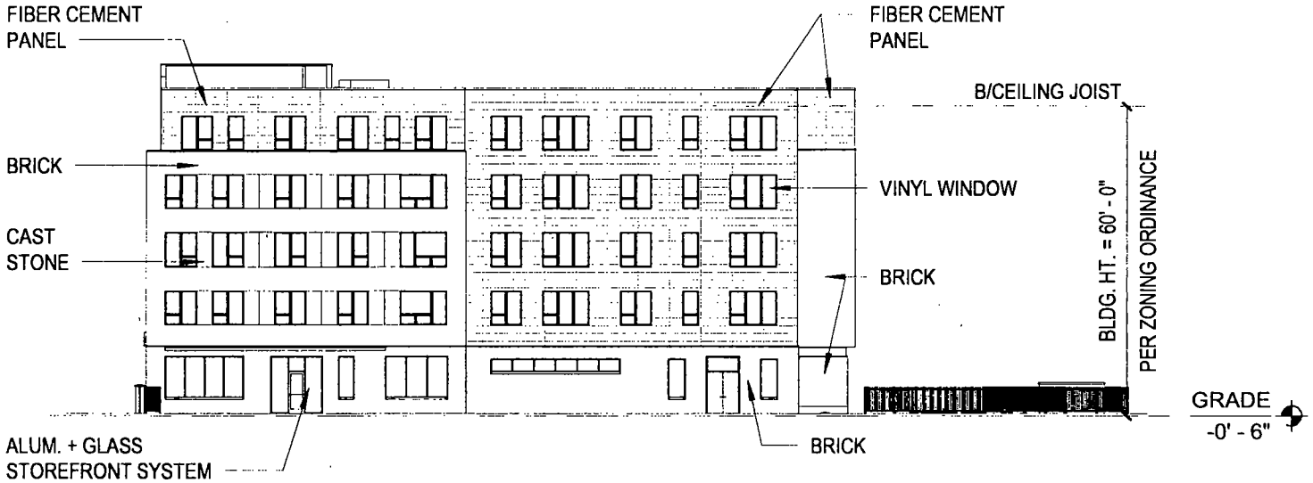
SOUTH ELEVATION
