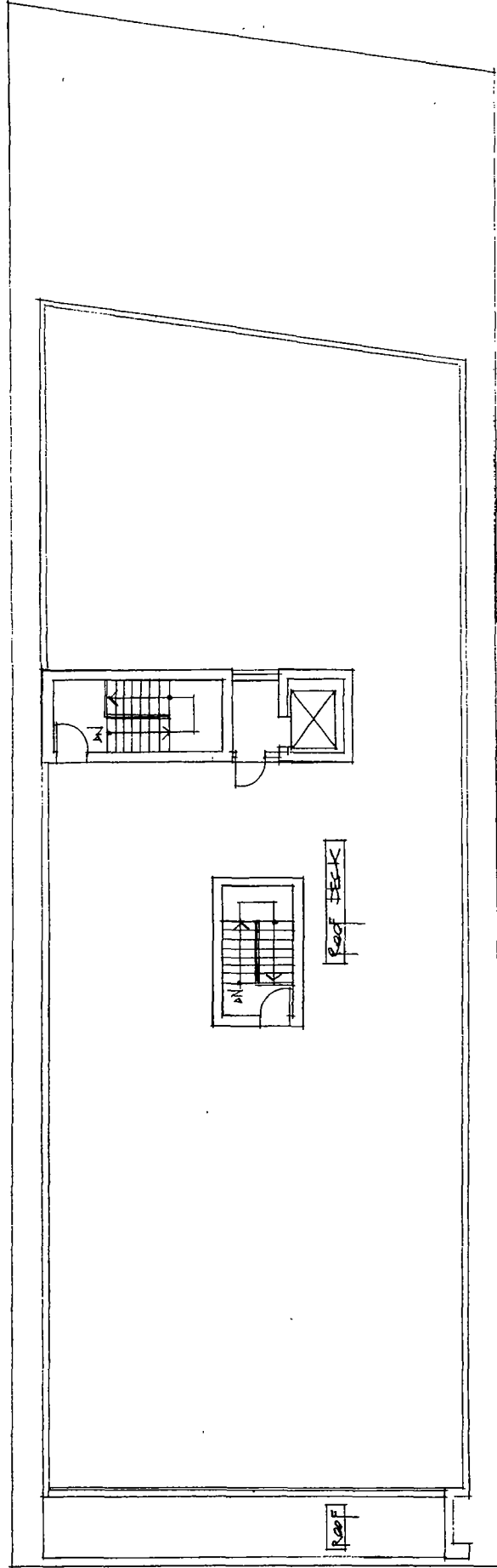
○ Roof Plan 1/8" = 1'-0"
