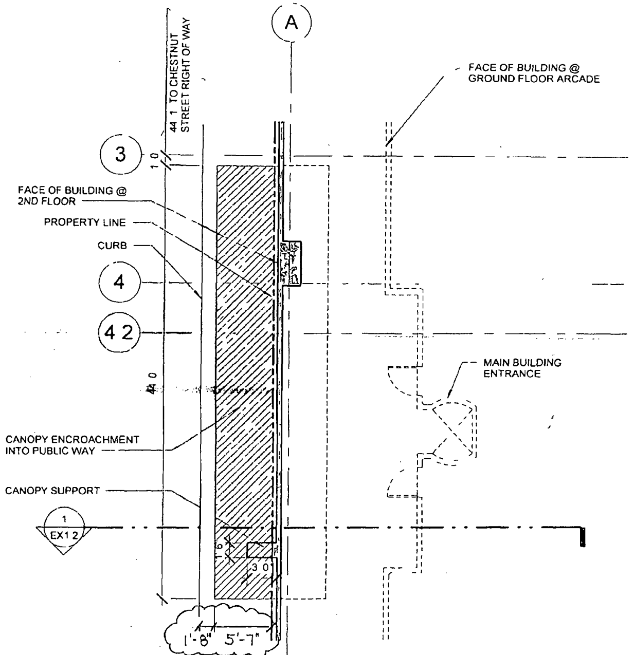
1 CANOPY PLAN SCALE 1/8" = 1'-0"
