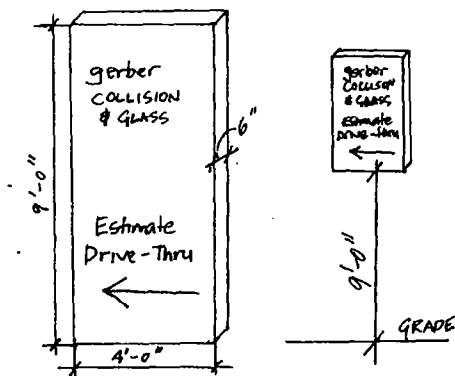
9'-0" x 4'-0" x 6" SIGN SCALE = 1/4" = 1'
