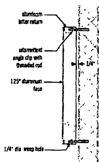
*AT&amp;T Letter Section Detail (typ)
