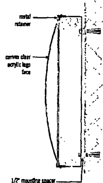
Globe Section Detail (typ)
