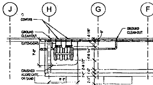
3 GI-1 SECTION NTS
