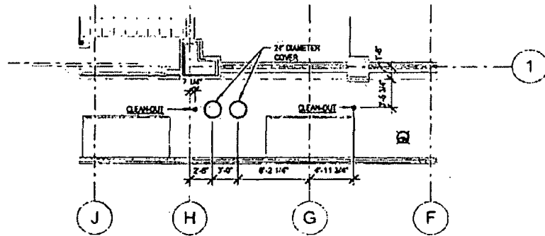
2 GI-1 FIRST FLOOR NTS
