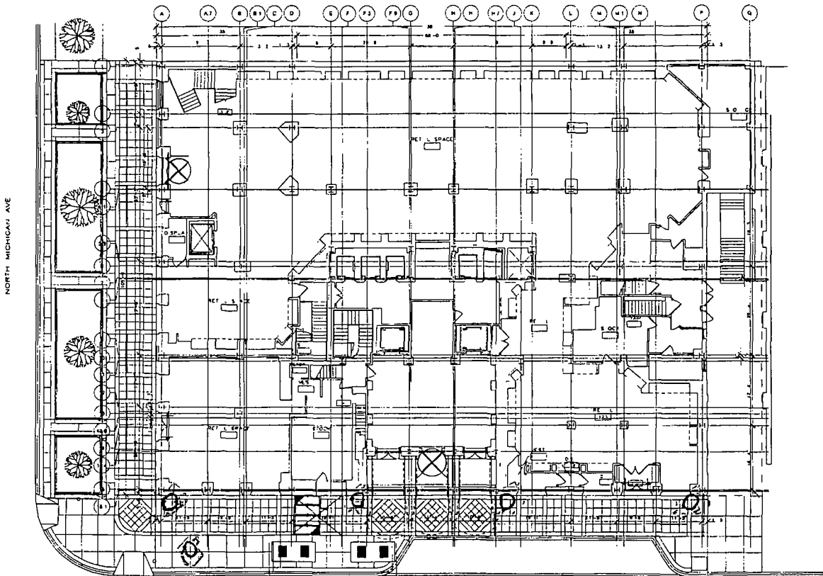
1 EXISTING GROUND FLOOR PLAN SCALE 1/16" = 1'-0"
