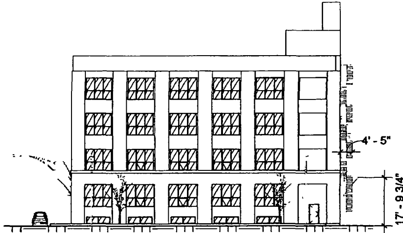
① PUBLIC WAY - FIRE ESCAPE 1/32" = 1'-0"
