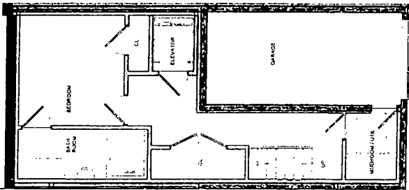
UNIT PRELIMINARY TYPE "A" FLOOR PLAN 1/8" = 1'-0"
