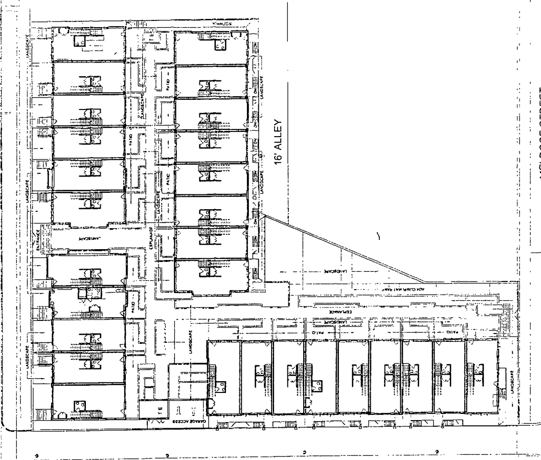
1. PRELIMINARY 1ST FLOOR 1/16" = 1'-0"
