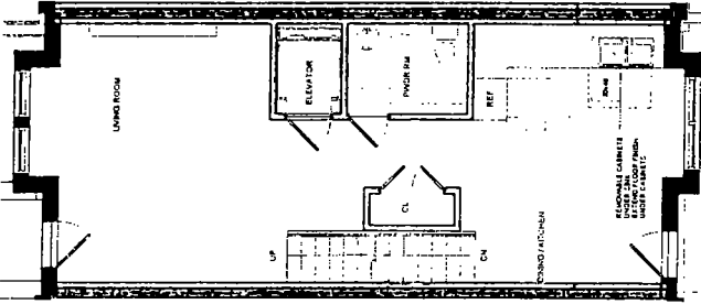
UNIT PRELIMINARY TYPE "A" 1ST FLOOR PLAN 1/8" = 1'-0"
