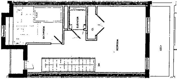
UNIT PRELIMINARY TYPE "A" 3RD FLOOR PLAN 1/8" = 1'-0"
