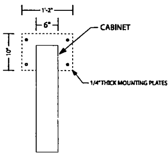
End View 1" = 1'-0"
