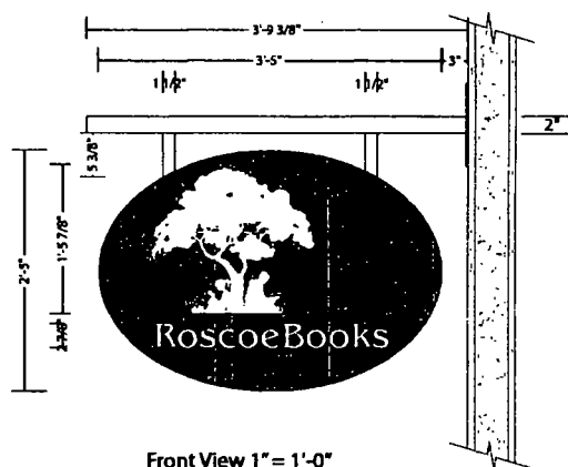
Front View 1" = 1'-0"
