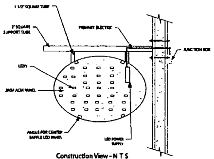
Construction View - N.T.S.
