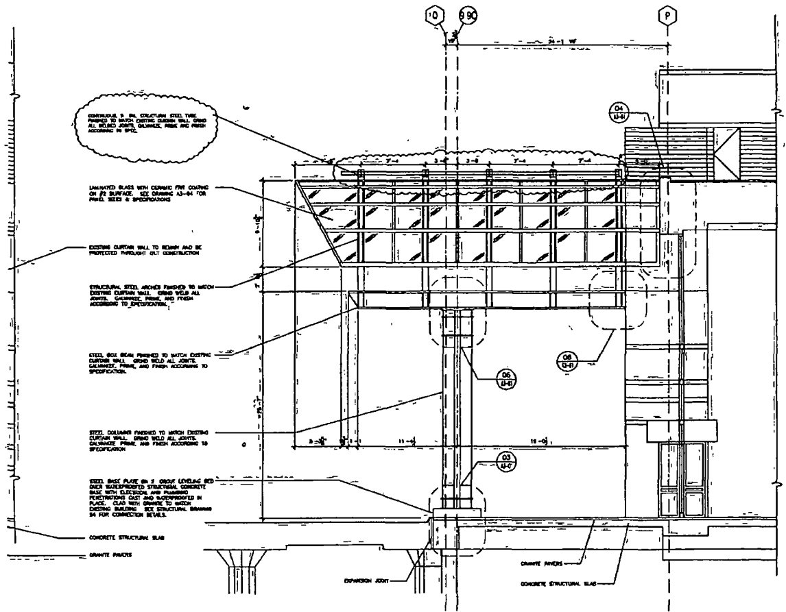
01 SOUTH CANOPY SECTION SCALE 1/2" = 1'-0"
