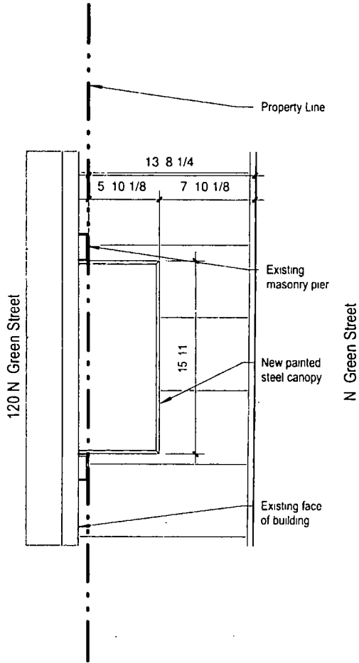
1 Canopy Roof Plan 1/8 = 1 0
