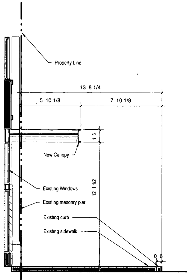
2 Canopy Section 1/4 = 1 0
