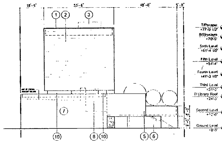
D. NORTH ELEVATION
