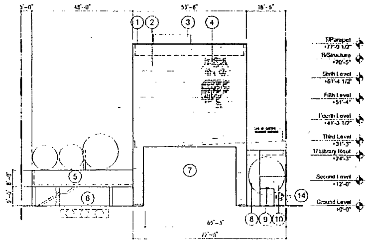
B. SOUTH ELEVATION
