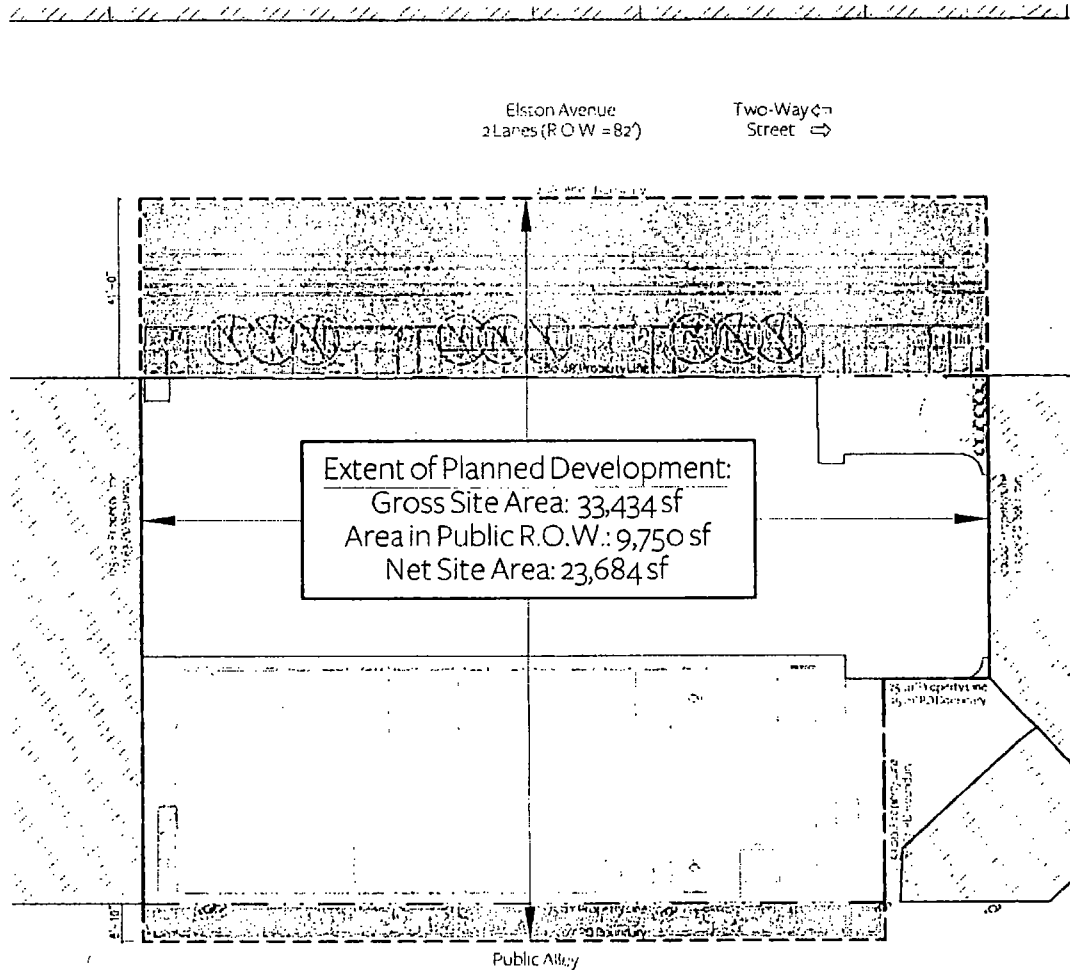
PLANNED DEVELOPMENT BOUNDARY LINE MAP
