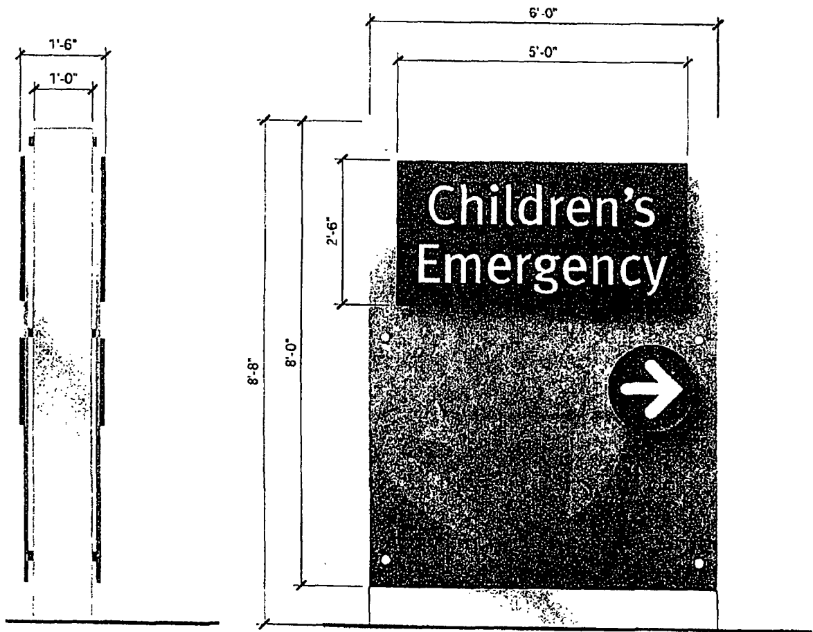
Side View 1/2"=1'-0"
