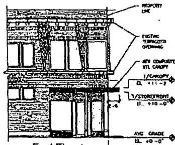
East Elevation
