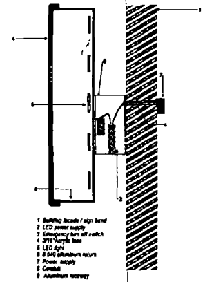
LED Raceway Mounting & SIDE VIEW
